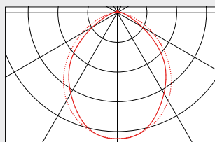
Wide beam 90°
