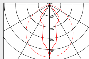
Narrow beam 30° clear
