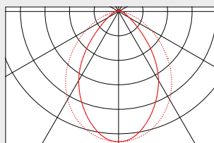
Deep beam 60°
