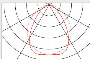
Medium beam 75°
