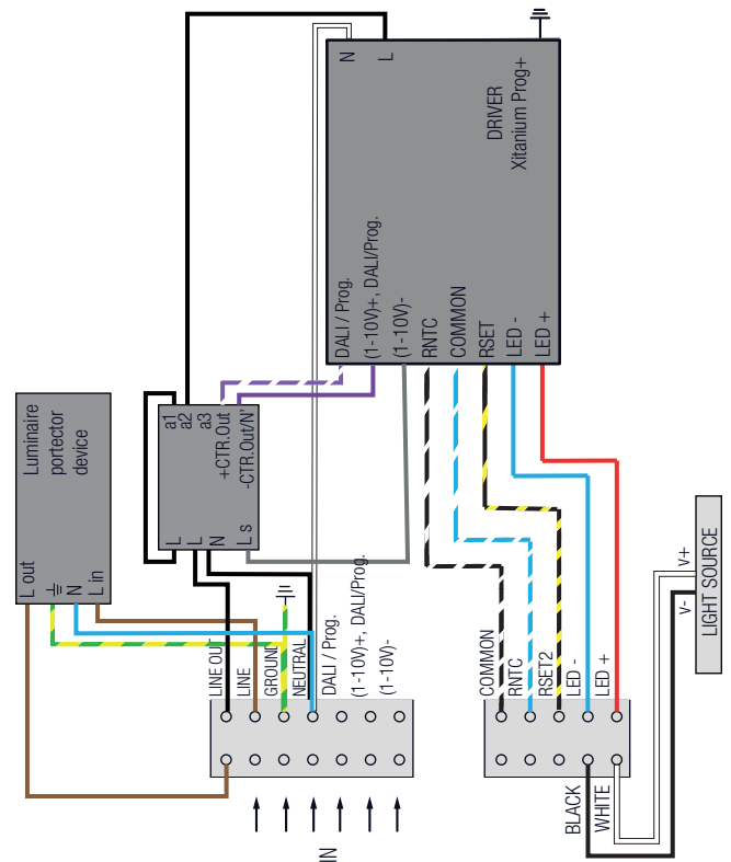
GUNNAR + SURGE PROTECTION DEVICE + IMCU + DRIVER PROG+
