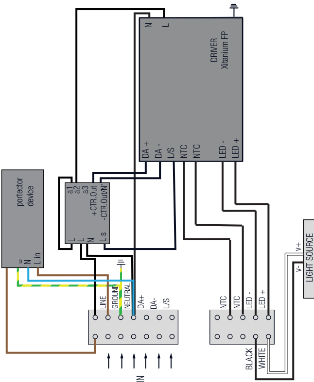
GUNNAR + SURGE PROTECTION DEVICE + IMCU + DRIVER FP
