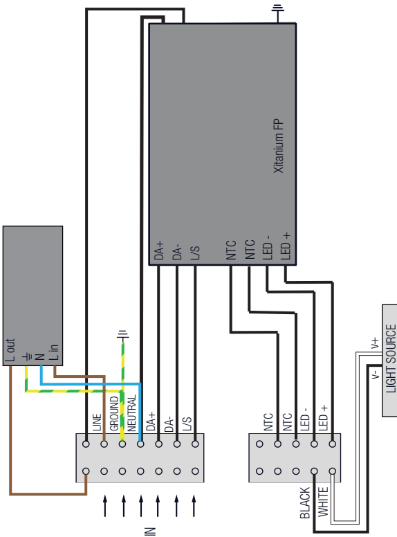
GUNNAR + SURGE PROTECTION DEVICE + DRIVER FP
