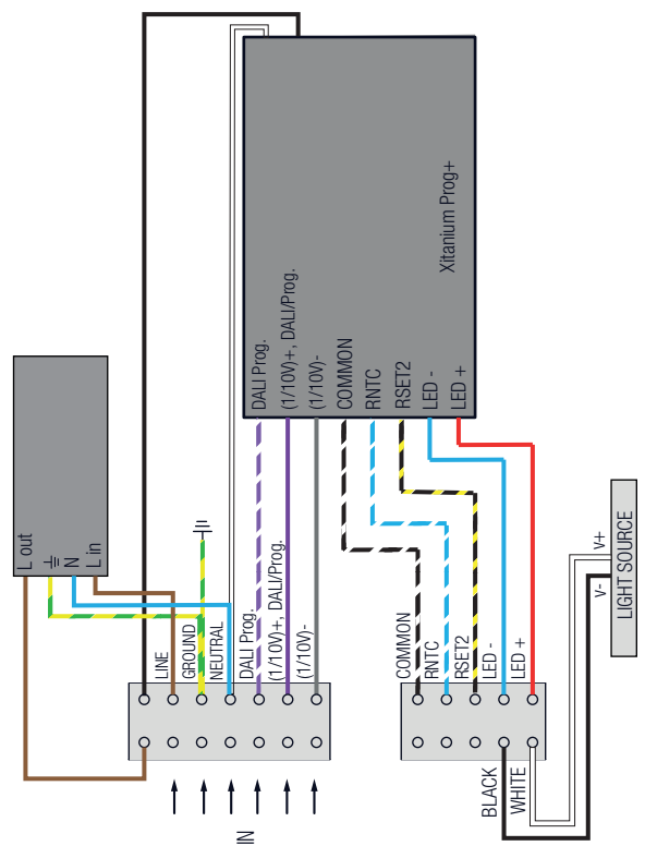
GUNNAR + SURGE PROTECTION DEVICE + DRIVER PROG+
